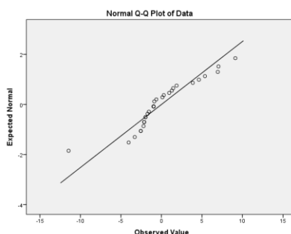
Gambar 1. Grafik Histogram Q-Q-Q Plot
